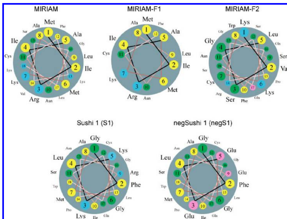
FIGURE 1: Peptides and peptide fragments. Helical wheel projection of the full-length (top) MIRIAM peptide and fragments MIR-F1 (left) and MIR-F2 (right). Helical wheel projections visualize the distribution of hydrophobic (yellow) and polar residues (green) with respect to the helical axis, illustrating the amphipathic structure of MIRIAM and MIR-F1. Basic and acidic residues are displayed in cyan and red, respectively.
